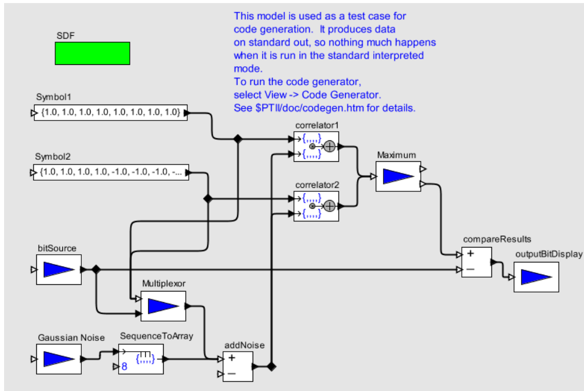
FIGURE 7.1. The Orthogonal Communication model, used as a Java code generation example.
