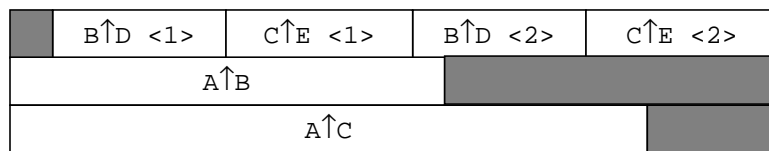
Buffer Period Lifetimes
