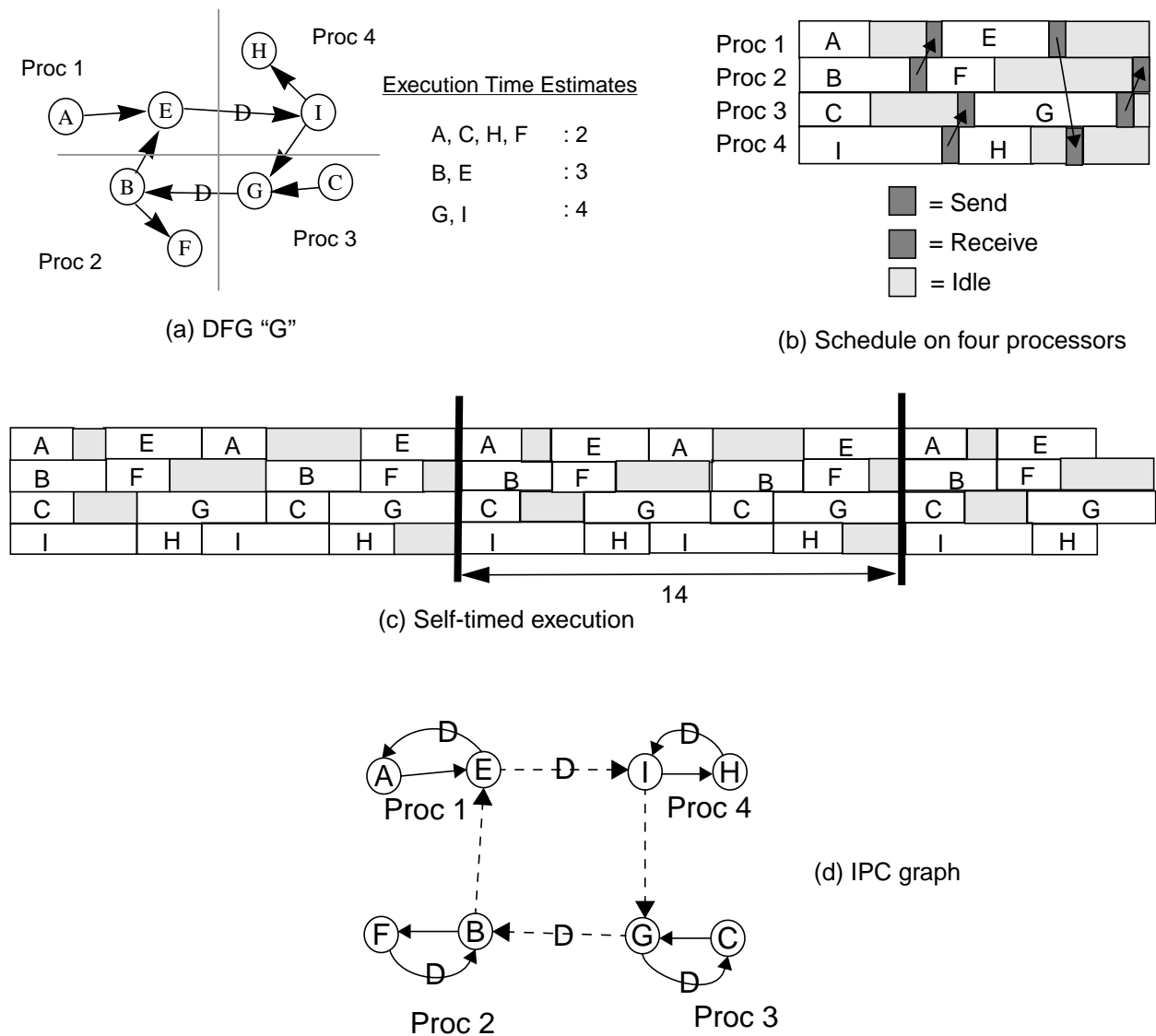
Figure 1. Self-timed execution.
