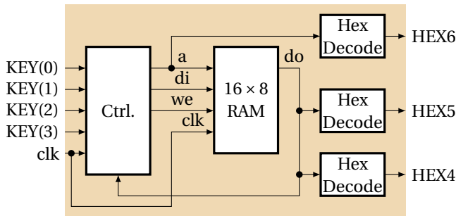
Figure 11: The block diagram of lab 1
