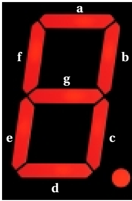
Figure 12: A seven-segment LED display. E.g., hex0(0) is a; hex0(6) is g
