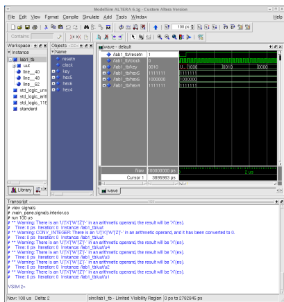
Figure 16: Running ModelSim and observing simulation results
