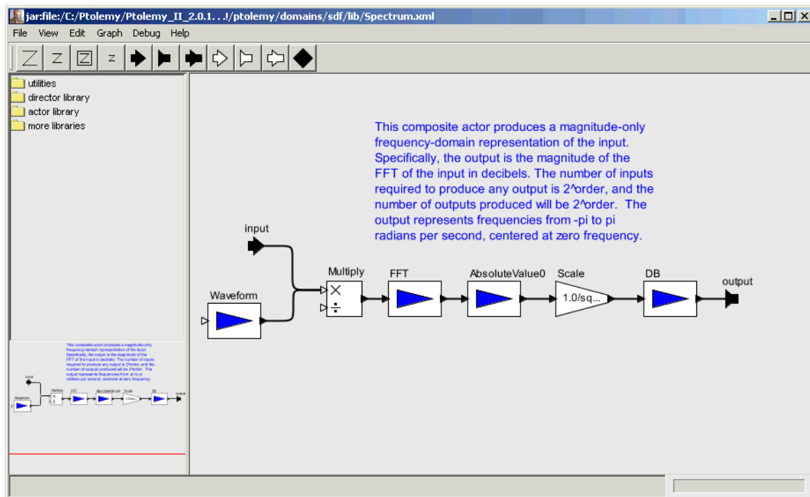
Figure 14.11 Vergil Screenshot.
