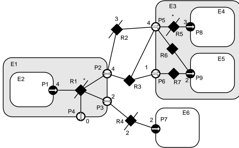
FIGURE 9.7. An example showing busses combined with input, output, and transparent ports.
