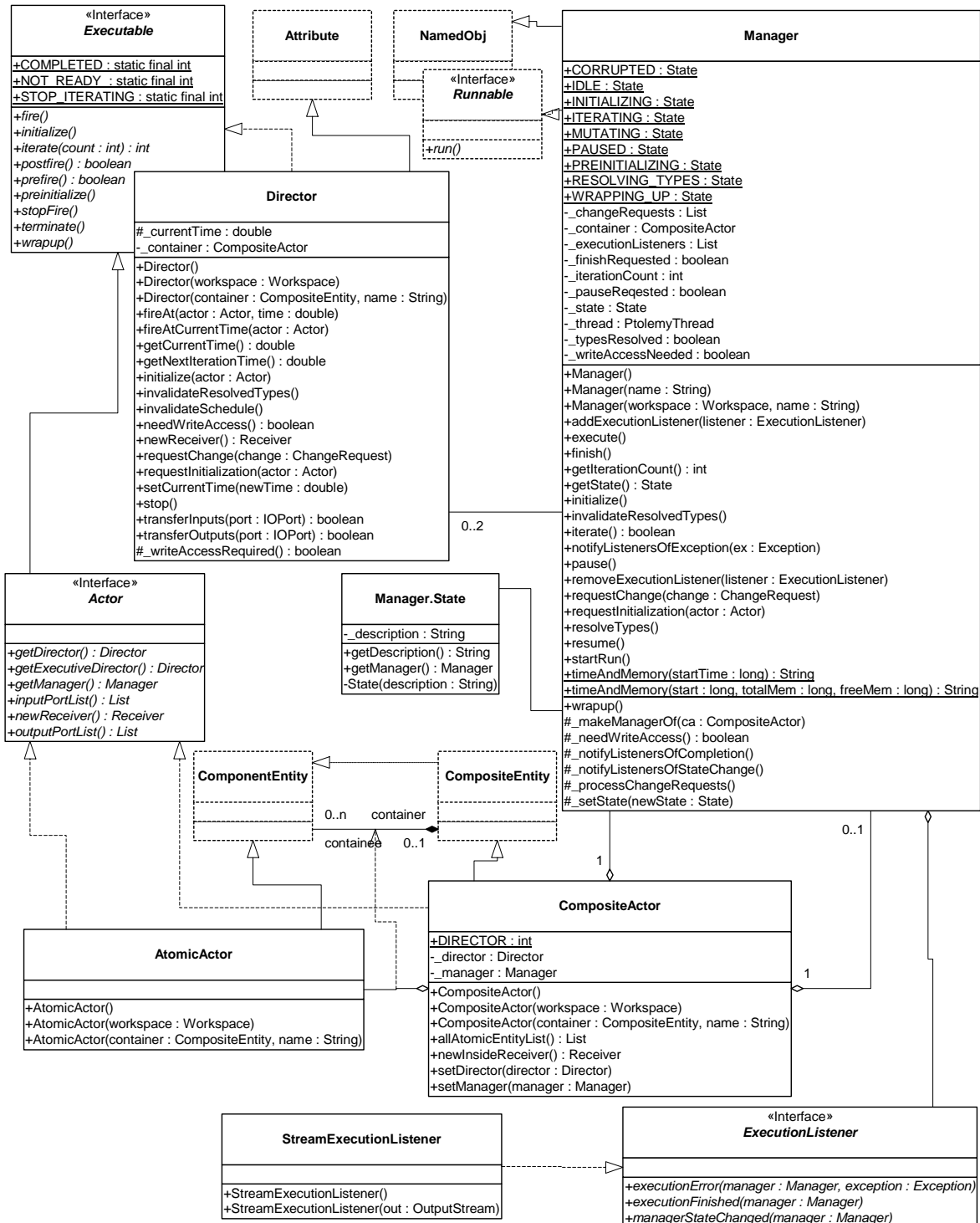
FIGURE 9.12. Basic classes in the actor package that support execution.
