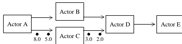
FIGURE 21.3. Timed deadlock (feedforward).
