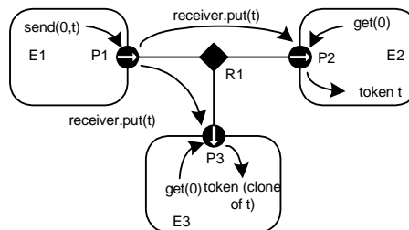
FIGURE 9.5. Channels may reach multiple destinations. This is represented by relations linking multiple input ports to an output port.
