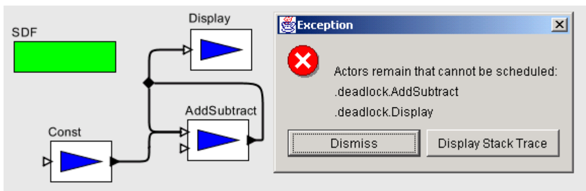
FIGURE 17.1. An SDF model that deadlocks.
