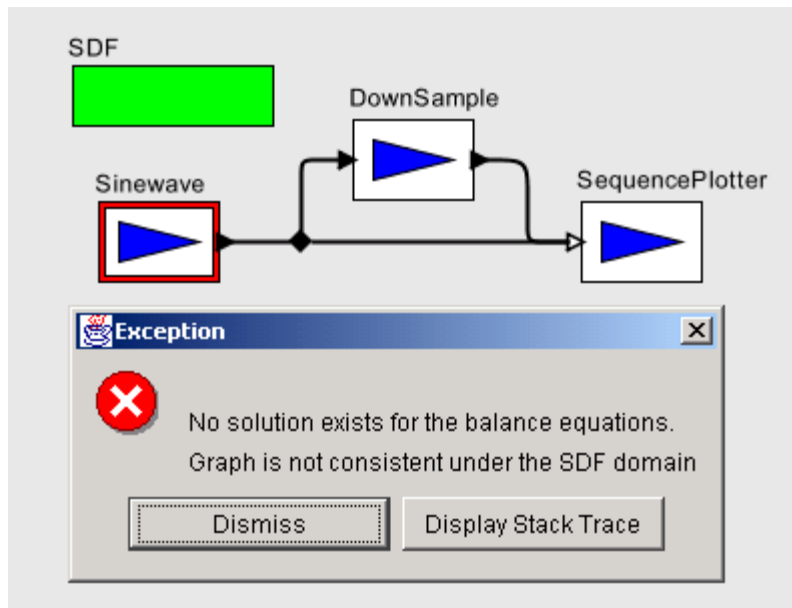
FIGURE 17.3. An SDF model with inconsistent rates.
