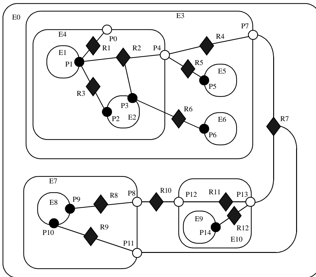
FIGURE 8.8. An example of a clustered graph.
