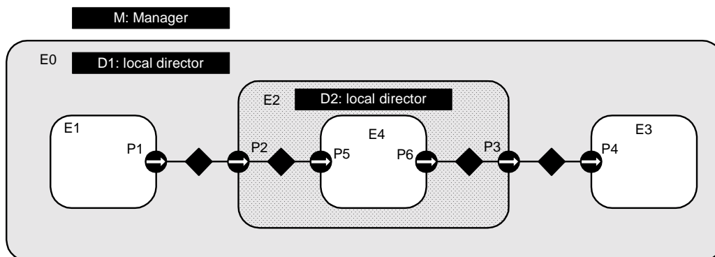
FIGURE 9.16. An example of an opaque composite actor. E0 and E2 both have local directors, not necessarily implementing the same model of computation.
