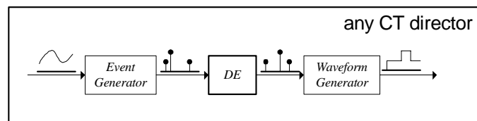
FIGURE 16.5. Embedding a DE component in a CT system.
