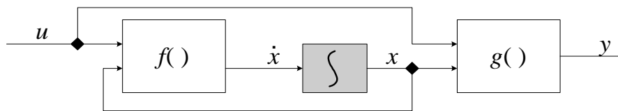
FIGURE 16.2. A conceptual block diagram for continuous time systems.
