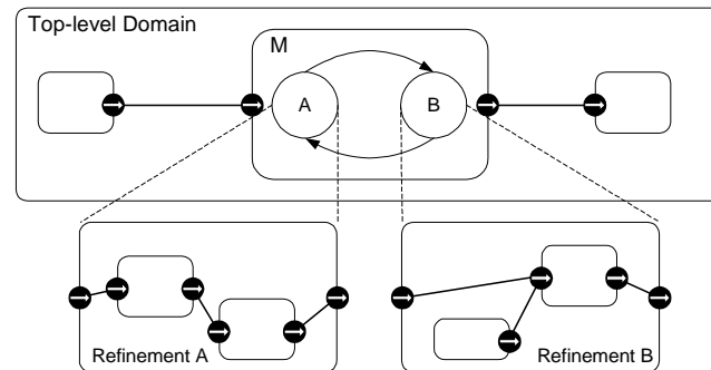
FIGURE 18.5. A modal model example.
