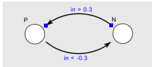
FIGURE 18.6. The mode controller for SchmidTrigger.
