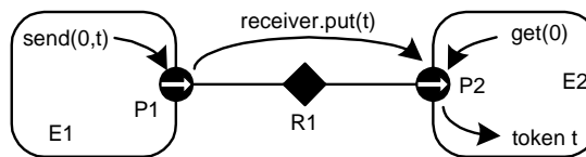
FIGURE 9.1. Message passing is mediated by the IOPort class. Its send() method obtains a reference to a remote receiver, and calls the put() method of the receiver, passing it the token t . The destination actor retrieves the token by calling the get() method of its input port.
