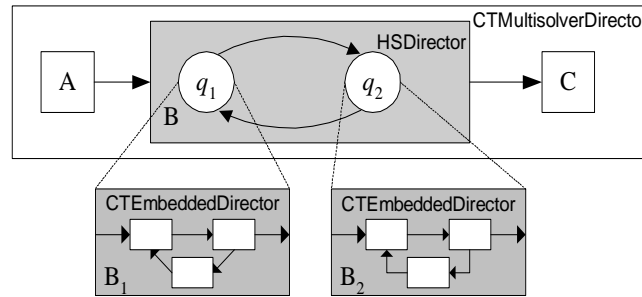
FIGURE 16.7. Hybrid system modeling.
