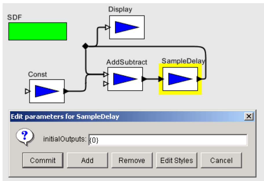
FIGURE 17.2. The model of figure 17.1 corrected with an instance of SampleDelay in the feedback loop.
