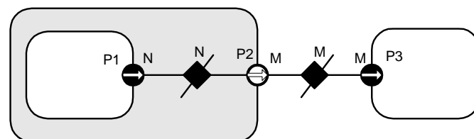
FIGURE 9.9. Bus widths inside and outside a transparent port need not agree..
