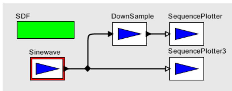
FIGURE 17.4. Figure 17.3 modified to have consistent rates.
