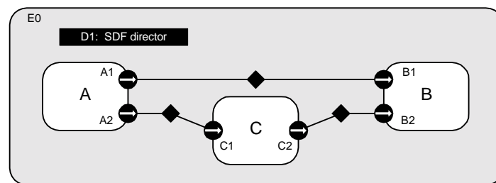
FIGURE 17.8. An example SDF model.
