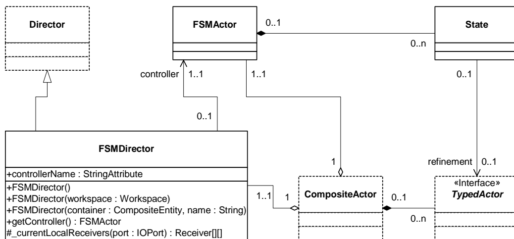
FIGURE 18.11. FSM kernel classes that support modal models.
