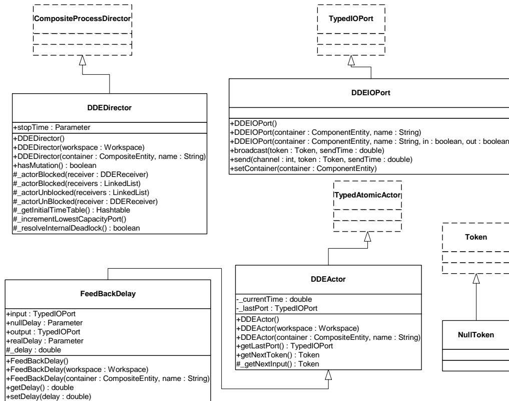
FIGURE 21.6. Additional classes in the DDE kernel.
