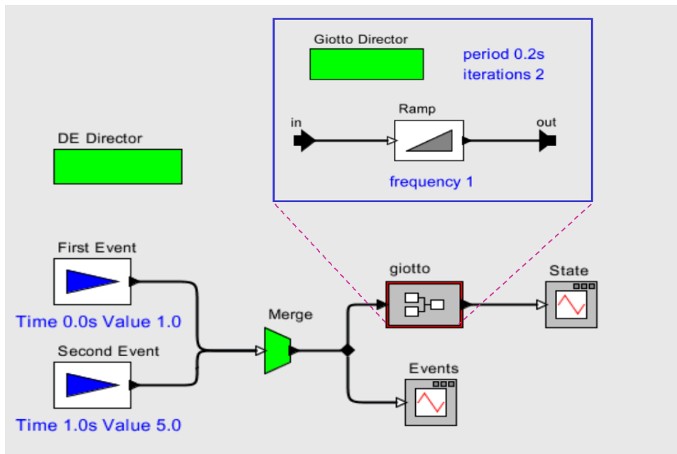
FIGURE 19.4. Giotto model embedded in DE model.
