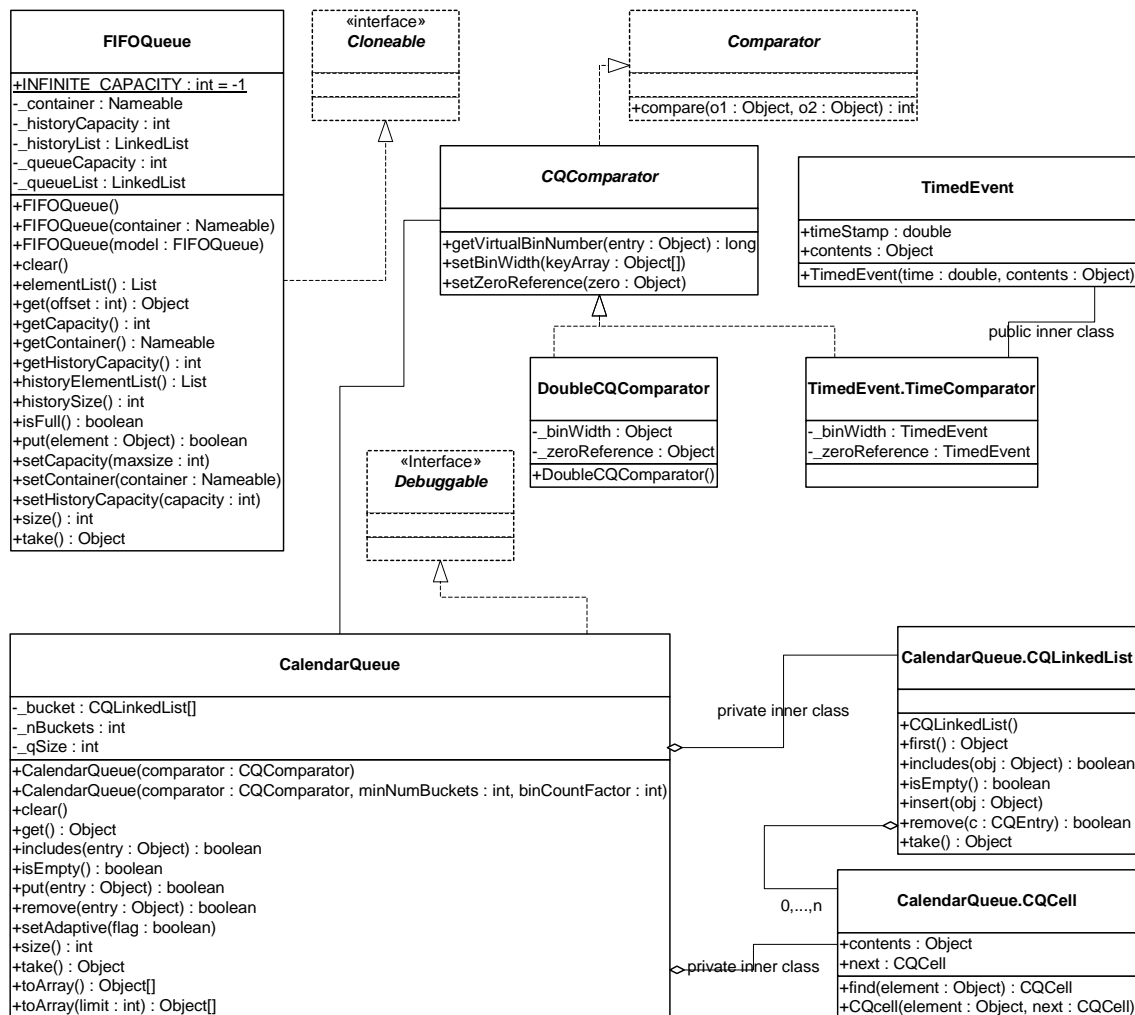
FIGURE 9.10. Static structure diagram for the actor.util package.
