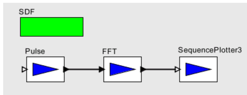
FIGURE 17.5. A model that plots the Fast Fourier Transform of a signal. Only one iteration must be executed to plot all 256 values of the FFT, since the FFT actor produces and consumes 256 tokens each firing.
