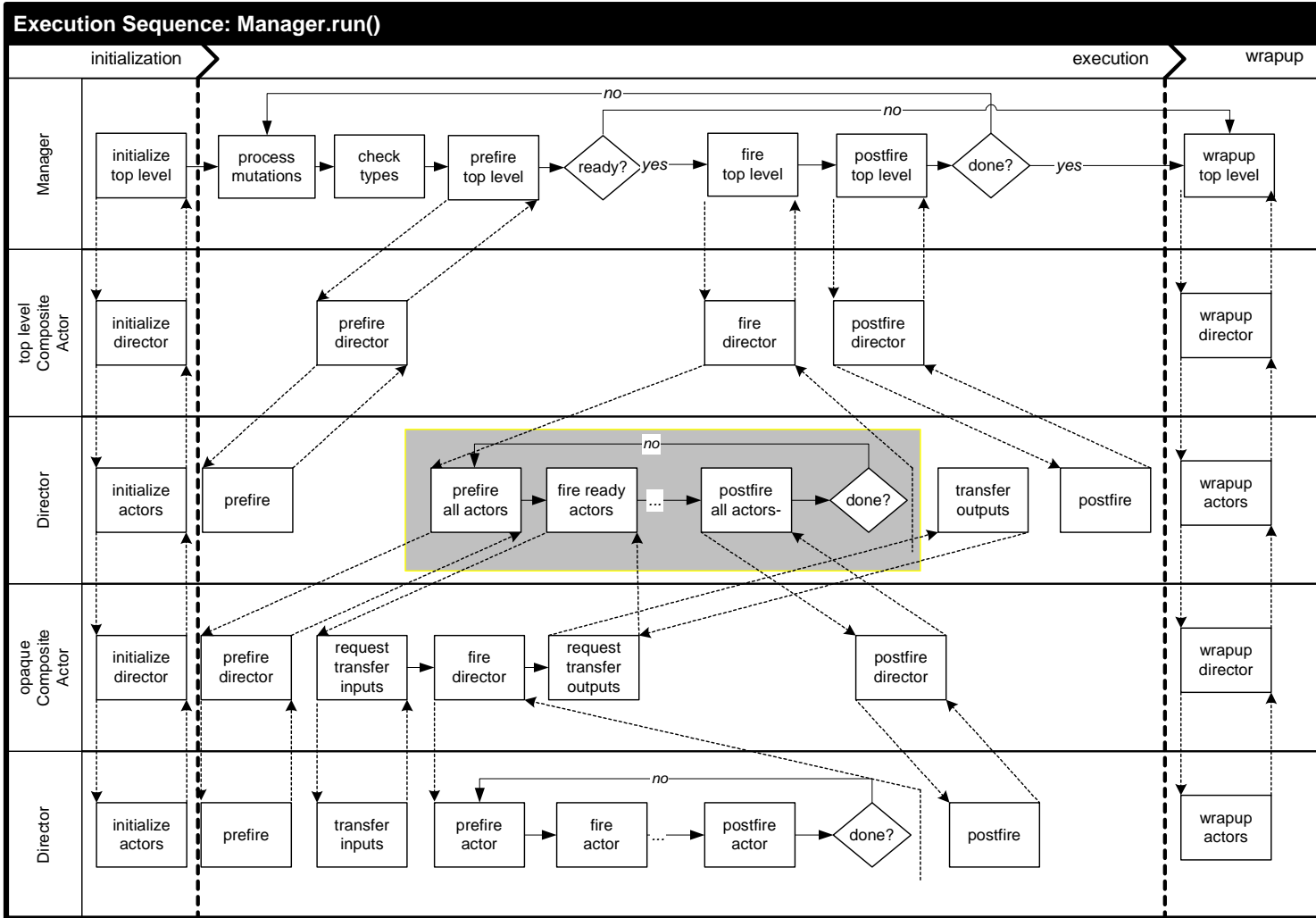
FIGURE 9.15. Alternative execution sequence implemented by run() method of the Director class.
