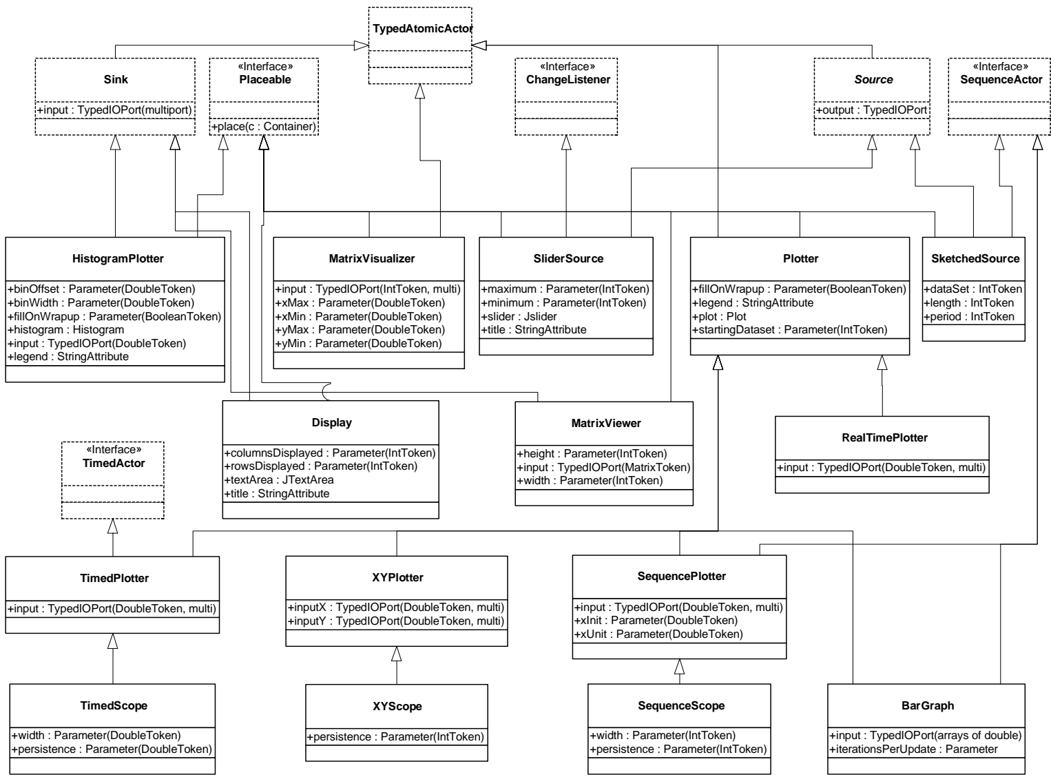
FIGURE 4.3. Organization of actors in the ptolemy.actor.lib.gui package.
