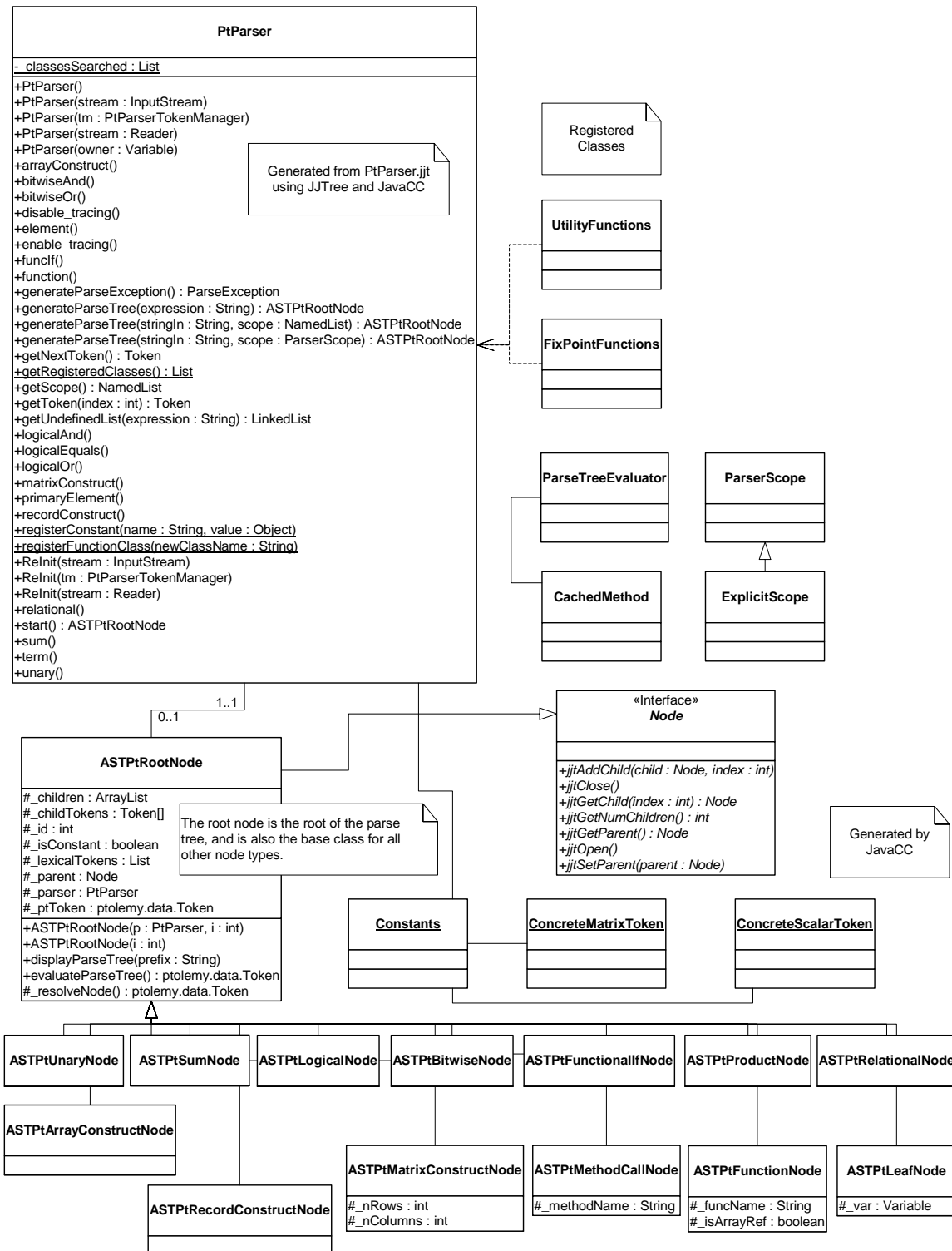
FIGURE 10.4. Static structure diagram for the parser classes in the data.expr package
