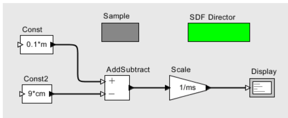
FIGURE 10.7. A model that uses the sample unit system.
