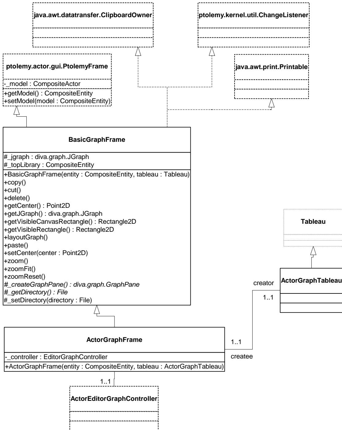
Figure 14.12 Static structure of the Ptolemy graph editor.
