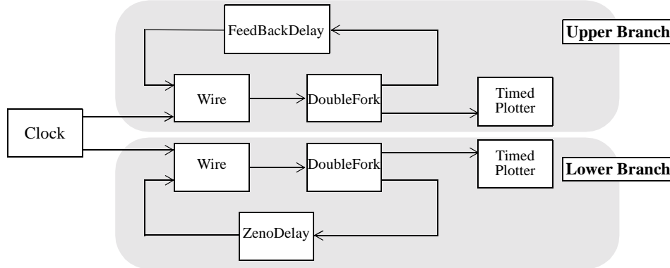
FIGURE 21.7. Localized Zeno condition topology.
