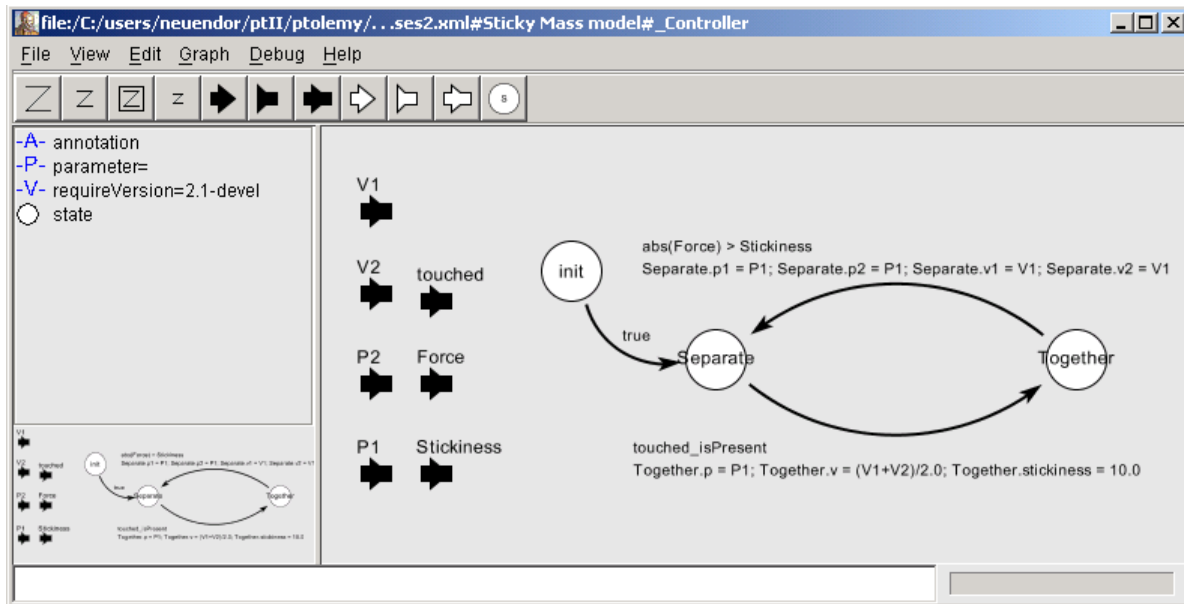
Figure 14.13 Vergil Screenshot.
