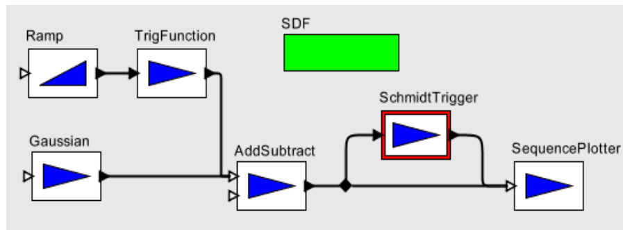
FIGURE 18.9. The top-level model with the SchmidtTrigger.
