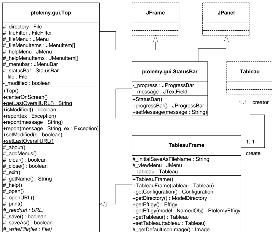
Figure 14.6 Static structure diagram for the TableauFrame class.
