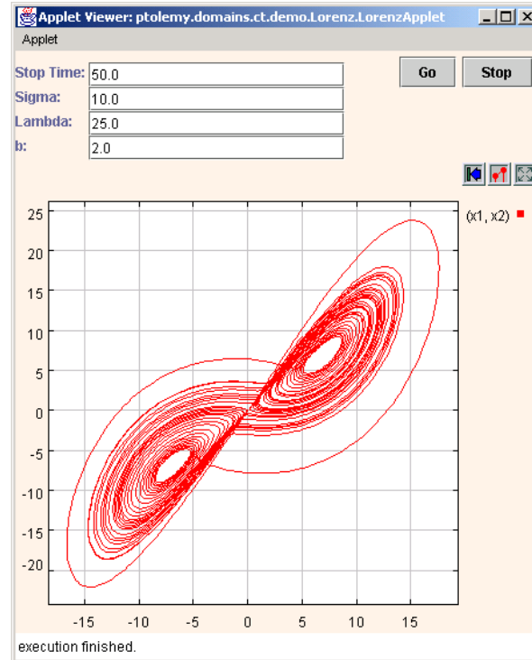
FIGURE 16.9. The simulation result of the Lorenz system.
