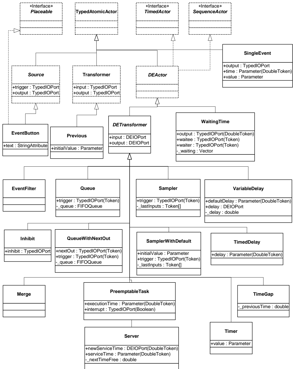
FIGURE 15.5. The library of DE-specific actors.
