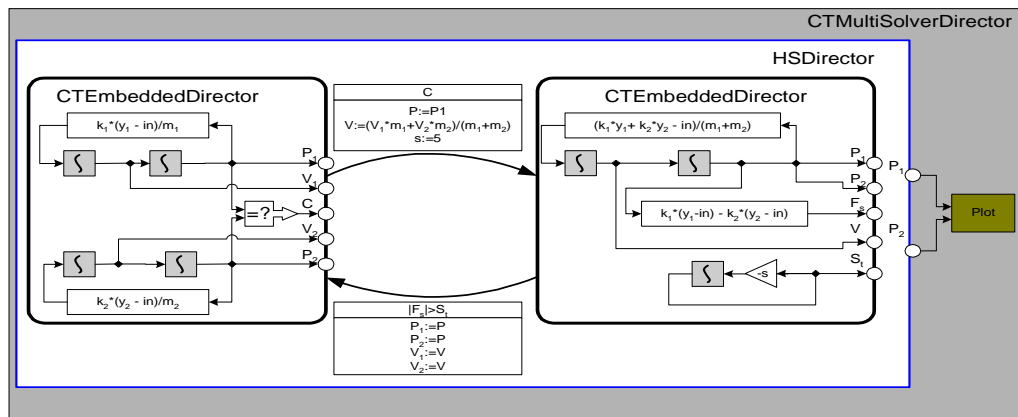
FIGURE 16.14. Modeling sticky point masses.
