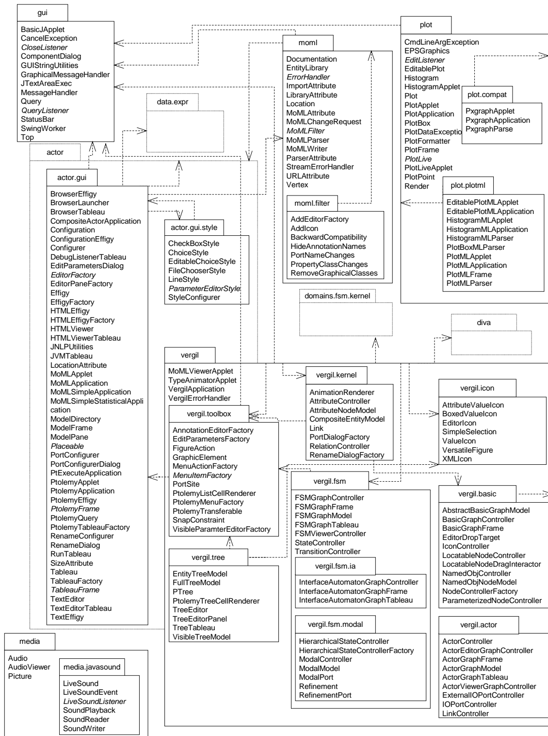
FIGURE I.9. Packages in Ptolemy II that support user interfaces, including the MoML XML schema and the Vergil visual editor.
