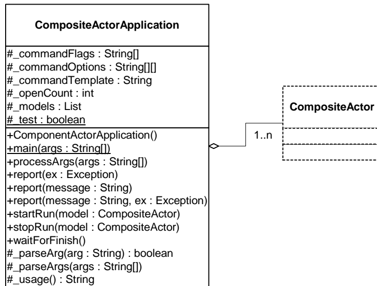
FIGURE 7.6. Any class that extends CompositeActor can be executed using the CompositeActorApplication class.
