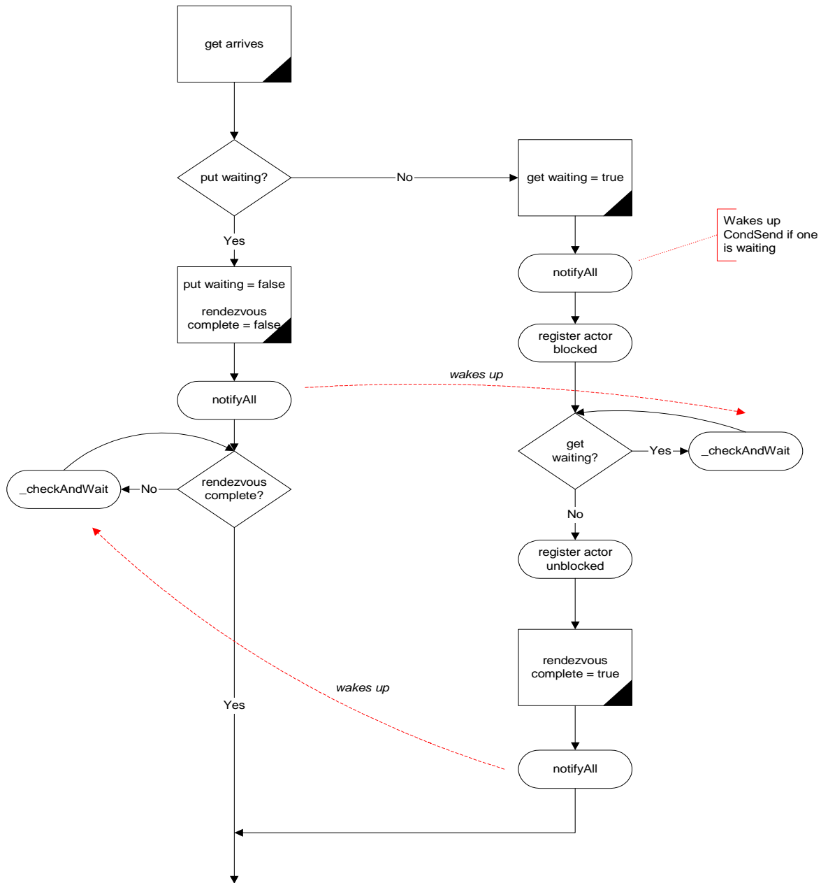
FIGURE 20.10. Rendezvous algorithm.
