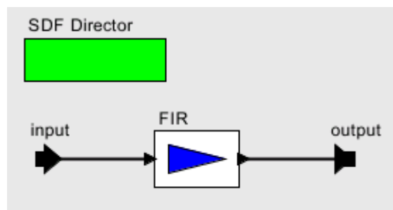
FIGURE 17.7. A model that implements a block FIR filter. The vectorizationFactor parameter of the director is set to the size of the block.
