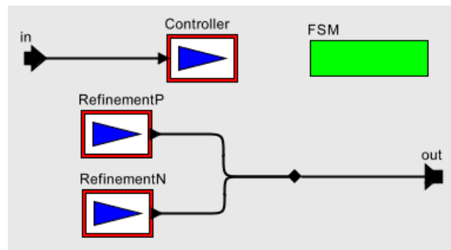
FIGURE 18.8. The SchmidTrigger modal model.
