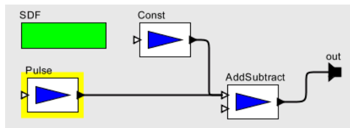
FIGURE 18.7. Model for the refinements in SchmidTrigger.
