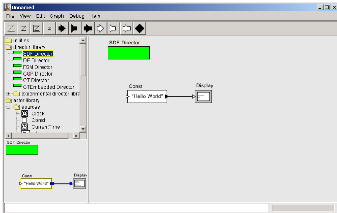
FIGURE 2.4. The Hello World example.
