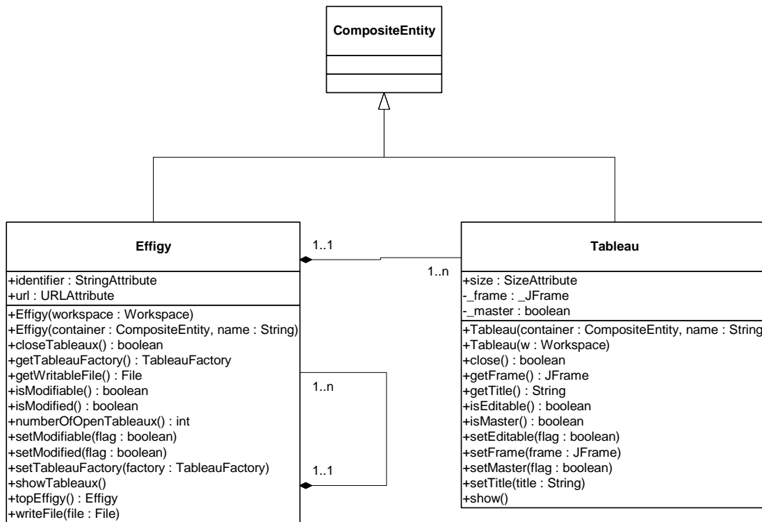
Figure 14.1 Static structure diagram for effigies and tableaux.
