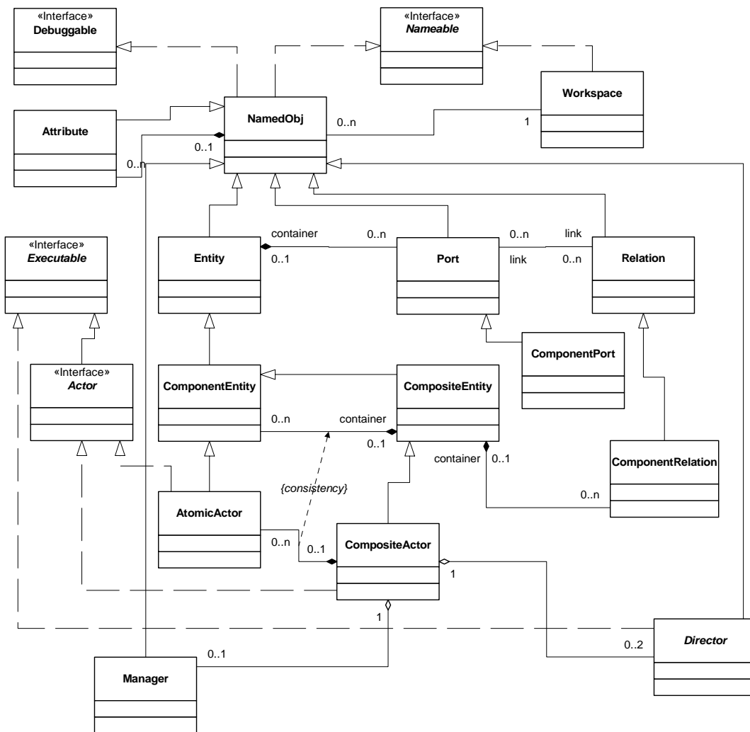
FIGURE 1.5. Some of the key classes in Ptolemy II. These are defined in the kernel , kernel.util , and actor packages. They define the Ptolemy II abstract syntax and abstract semantics.
