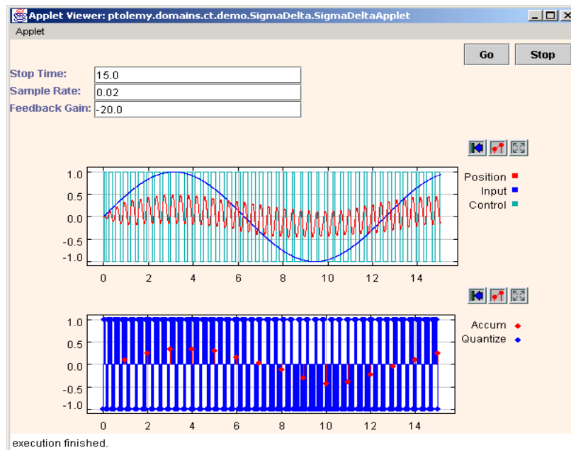
FIGURE 16.12. Execution result of the microaccelerometer system.
