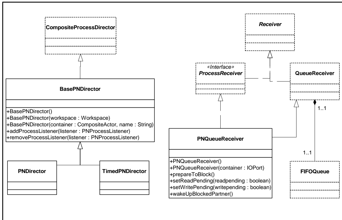
FIGURE 22.1. Static structure of the PN kernel.
