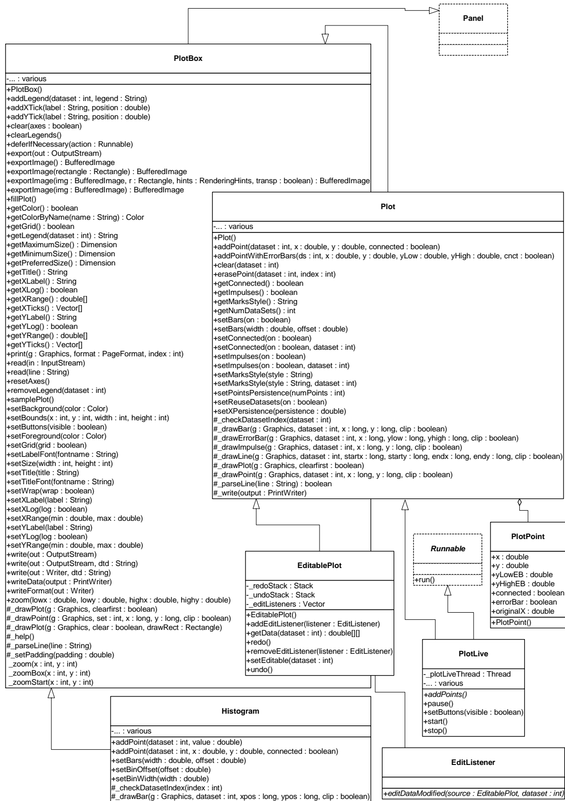
FIGURE 13.6. The core classes of the plot package.
